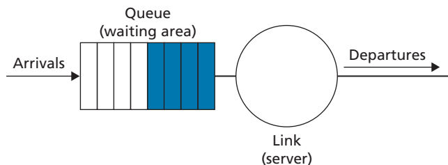
Figure 4.11 ♦ FIFO queuing abstraction
